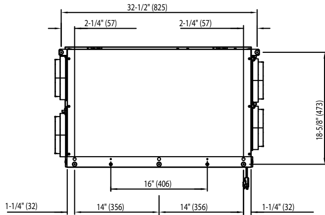
Hanging Hole Pattern (Bracket) Top View
